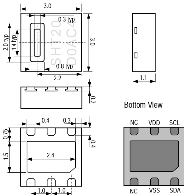
Figure 1: Drawing of SHT20 sensor package, dimensions are given in mm (1mm = 0.039inch), tolerances are \pm 0.1 mm. NC and die pad (center pad) are internally connected to VSS. They may be left floating. VSS = GND, SDA = DATA. Numbering of E/O pads starts at lower right corner (indicated by notch in die pad) and goes clockwise (compare Table 2).
