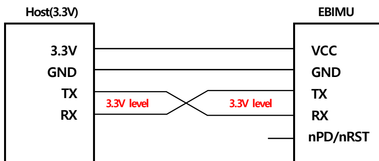
3.3V interface
