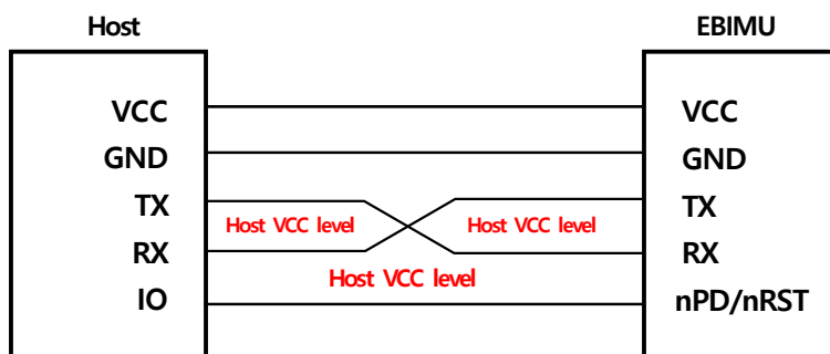
nPD/nRST connection
