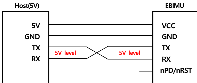
5V interface
