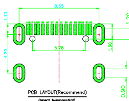
PCB LAYOUT(Recommend) (General Temperature:0~85℃)
