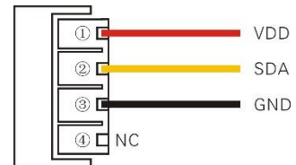
Figure 6. AM2305B Wiring Diagram
