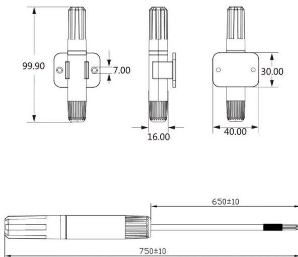
Figure 13. sensor encapsulation (unit: mm ; not specified tolerance: ± 0.2 mm)
