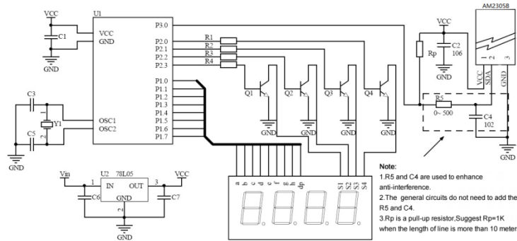
Figure 7. CM2305B One-Wire Application Circuitry
