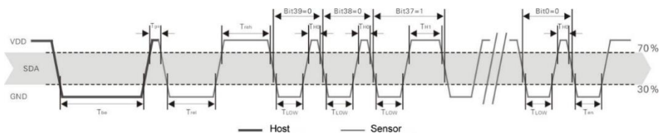
Figure 9. CM2305B Single bus communication timing
