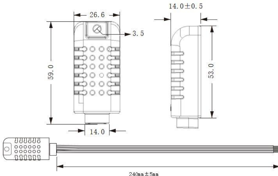
Figure 12. CM2301B sensor encapsulation (unit: mm not specified tolerance: ± 0.2 mm)
