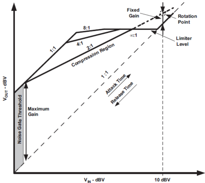
Figure 35. Output Signal vs. Input Signal State Diagram
